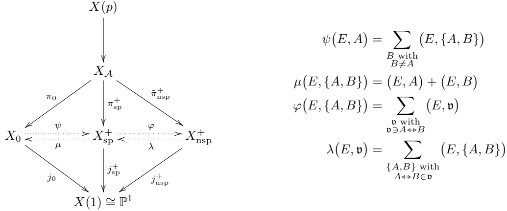
Figure 1: The various maps in Chen's theorem
