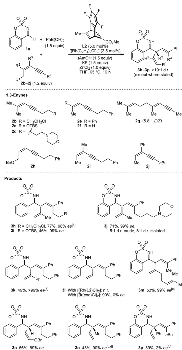
Scheme 3. Variation of the 1,3-enyne. See the footnote of Scheme 2 for general considerations. [a] Using 1.5 equiv of 1,3-enyne 2b . [b] Using 3.0 equiv each of PhB(OH) 2 and t AmOH. [c] Using 1.5 equiv of 1,3-enyne 2g and 2.0 equiv each of PhB(OH) 2 , KF, and t AmOH. [d] An 8.2:1 inseparable mixture of 3o and the imine phenylation product was obtained (the yield of 3o has been adjusted accordingly).
