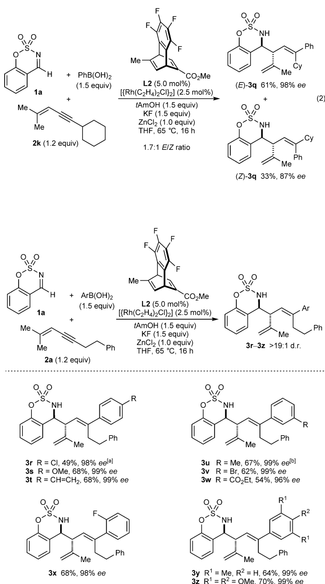
Scheme 4. Variation of the arylboronic acid. See the footnote of Scheme 2 for general considerations. [a] Isolated in approximately 91% purity (the yield has been adjusted accordingly). [b] Using 1.5 equiv of 1,3-enyne 2a .
