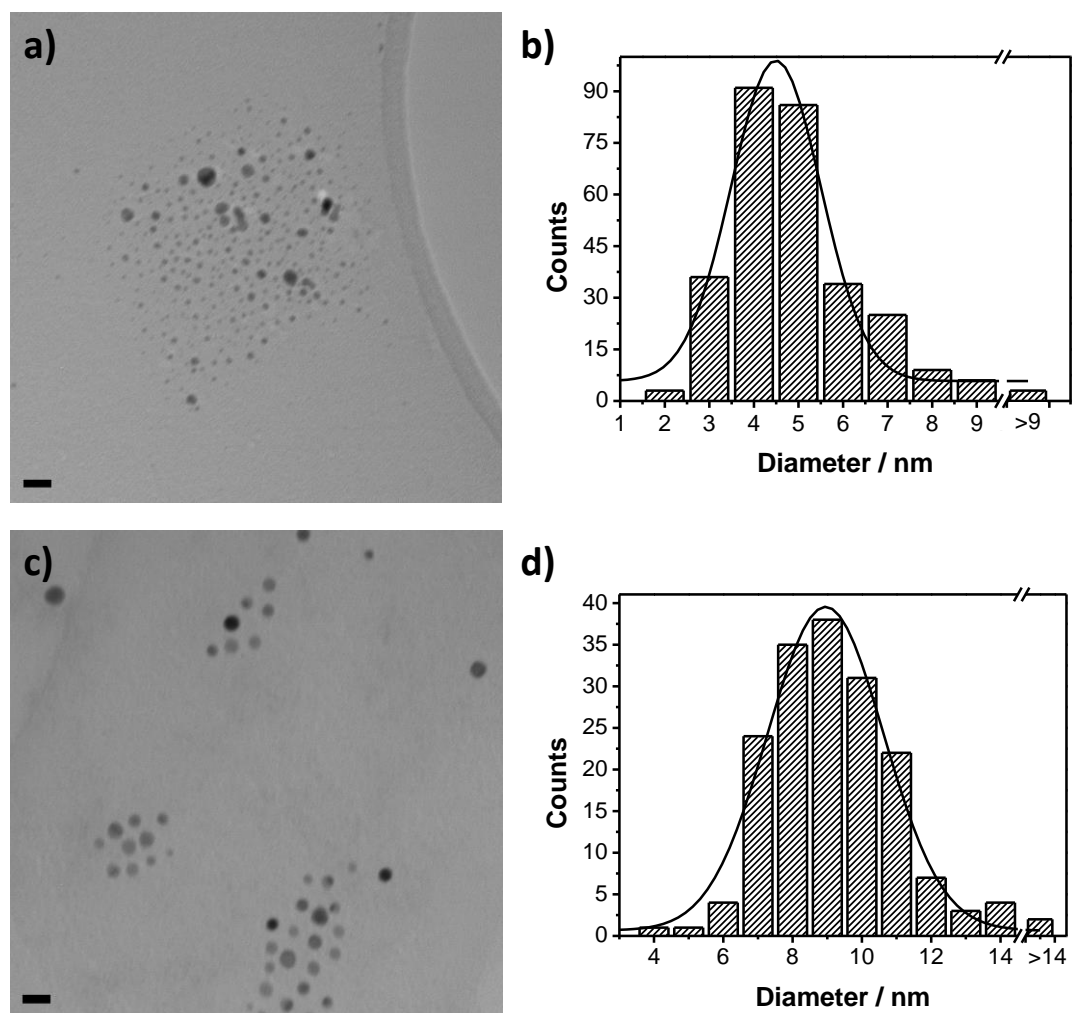
Figure 3. Transmission electron micrographs ( a and c ) and size distribution histograms ( b and d ) of: a and b ) PR-AuNP-PEG (biphasic) ( n = 298 ) and c and d ) PR-AuNP-PEG (monophasic) ( n = 172 ). Scale bars: 20 nm.
