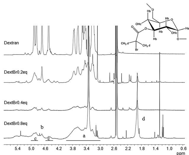
Fig. 2 1 H-NMR spectra of dextran and dextran macroinitiators (dextBr0.2 eq., dextBr0.4 eq. and dextBr0.8 eq.) in DMSO- d 6 .
