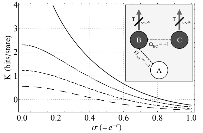
FIG. 1. The QSS secure key rate K , Eq. (15), is plotted against the squeezing r of a 3-mode noisy Gaussian cluster state, obtained from a pure state [20] \hat{U}_{AB}\hat{U}_{BC}|r\rangle_A|r\rangle_B|r\rangle_C , with \hat{U}_{ij} = \exp(\Omega_{ij}\hat{x}_i\hat{x}_j) , after Bob and Charlie's modes undergo individual pure-loss channels (i.e., quantum-limited attenuating channels), each modelled by a beam splitter with transmissivity T and zero excess noise (see inset). From top to bottom, the curves correspond to T = 1, 0.95, 0.9, 0.85 . All parties are assumed to be performing homodyne measurements of \hat{x}_i, \hat{p}_i , with i = A, B, C . The current experimentally accessible squeezing is limited to r \lesssim 1.15 (10dB), or \sigma \gtrsim 0.32 [57, 58], in which regime a nonzero K is still guaranteed for sufficiently large T , demonstrating the feasibility of our scheme.
