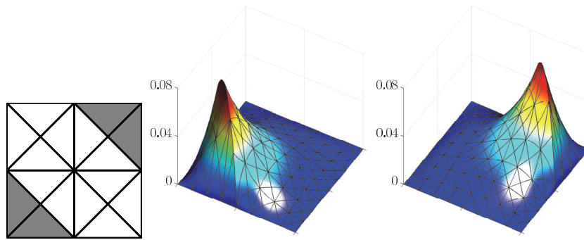
FIG. 1. Example from section 4.5: The initial mesh \mathcal{T}_0 (left) and the triangles T_f (bottom left) and T_g (top right) are indicated in gray. Shown is an approximation to the primal solution (middle) and dual solution (right) on a uniform mesh with 256 elements, where the singularities of both are clearly visible.
