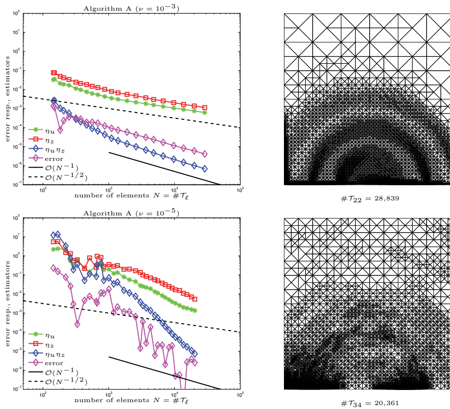
FIG. 6. Example from section 5.5: To study the robustness of the goal-oriented algorithm with respect to the diffusion coefficient \nu = 10^{-3} (top) and \nu = 10^{-5} (bottom), we plot \eta_{u,\ell} , \eta_{z,\ell} , and \eta_{u,\ell}\eta_{z,\ell} , as well as the goal error |N_z(u) - N_{z,\ell}(U_\ell)| , as output of Algorithm A with \theta = 0.6 over the numbers of elements \#\mathcal{T}_\ell (left). We show some related discrete meshes with > 20,000 elements (right).
