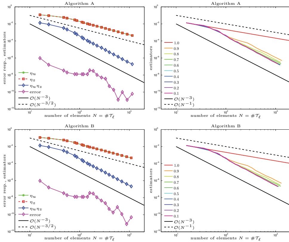
FIG. 2. Example from section 4.5: Estimators \eta_{u,\ell} and \eta_{z,\ell} , estimator product \eta_{u,\ell}\eta_{z,\ell} , and goal error |g(u) - g(U_\ell)| as output of Algorithms A–B with \theta = 0.5 (left), resp., estimator product for various \theta \in \{0.1, \dots, 0.9\} as well as for \theta = 1.0 , i.e., uniform mesh-refinement (right).
