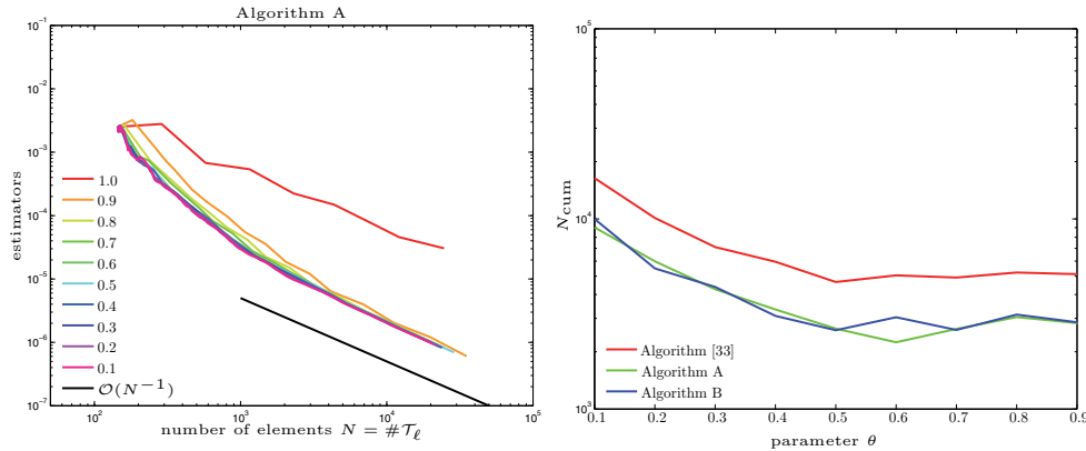
FIG. 5. Example from section 5.5 for p = 1 and \nu = 10^{-3} : Estimator product as output of Algorithm A for various \theta \in \{0.1, \dots, 0.9\} as well as for \theta = 1.0 , i.e., uniform refinement (left) and cumulative number of elements N_{\text{cum}} := \sum_{j=0}^{\ell} \#\mathcal{T}_j necessary to reach a prescribed accuracy \eta_{u,\ell} \eta_{z,\ell} \leq 10^{-4} over \theta \in \{0.1, \dots, 0.9\} .
