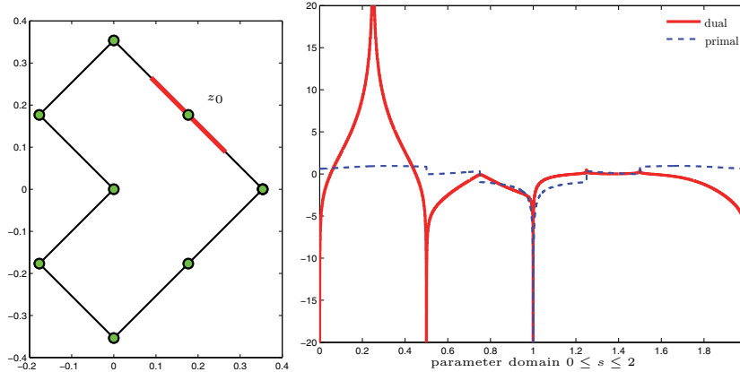
FIG. 7. Example from section 6.5: Domain \Omega with initial triangulation \mathcal{T}_0 (left) and the primal and dual solutions plotted over the arc-length (right), where s = 1 (resp., s = 0.25 ) corresponds to the reentrant corner (resp., z_0 ).
