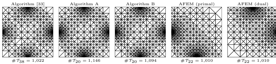
FIG. 3. Example from section 4.5: Meshes generated by goal-oriented algorithms as well as standard (nongol-oriented) AFEM driven by the primal error estimator (resp., the dual error estimator) for \theta = 0.5 .
