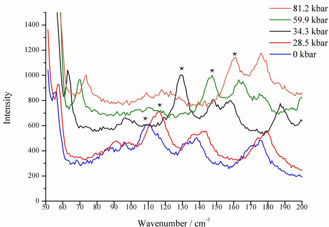
Figure 5. Variation in the \nu(\text{Au}_2) stretching frequency (identified by an asterisk) with increasing pressure.
