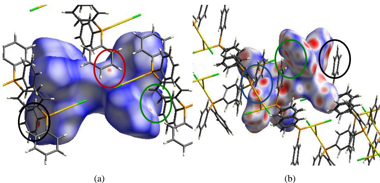
Figure 3. Hirshfeld surface of 1 at (a) ambient pressure and (b) 106.2 kbar. Red areas: contacts which are shorter than the sum of the van der Waals radii; white areas: contacts which are short but non-overlapping; blue areas: contacts which are longer than the sum of the van der Waals radii. The coloured circles represent the different types of interaction: \pi \cdots \pi (black); C-H \cdots \pi (green); \pi \cdots C-H (red); H \cdots H (blue).
