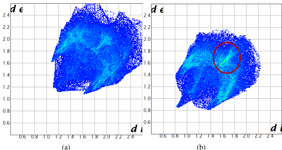
Figure 4. Fingerprint plots of a molecule of 1 at (a) ambient pressure and (b) 106.2 kbar, showing all the intermolecular interactions present.
