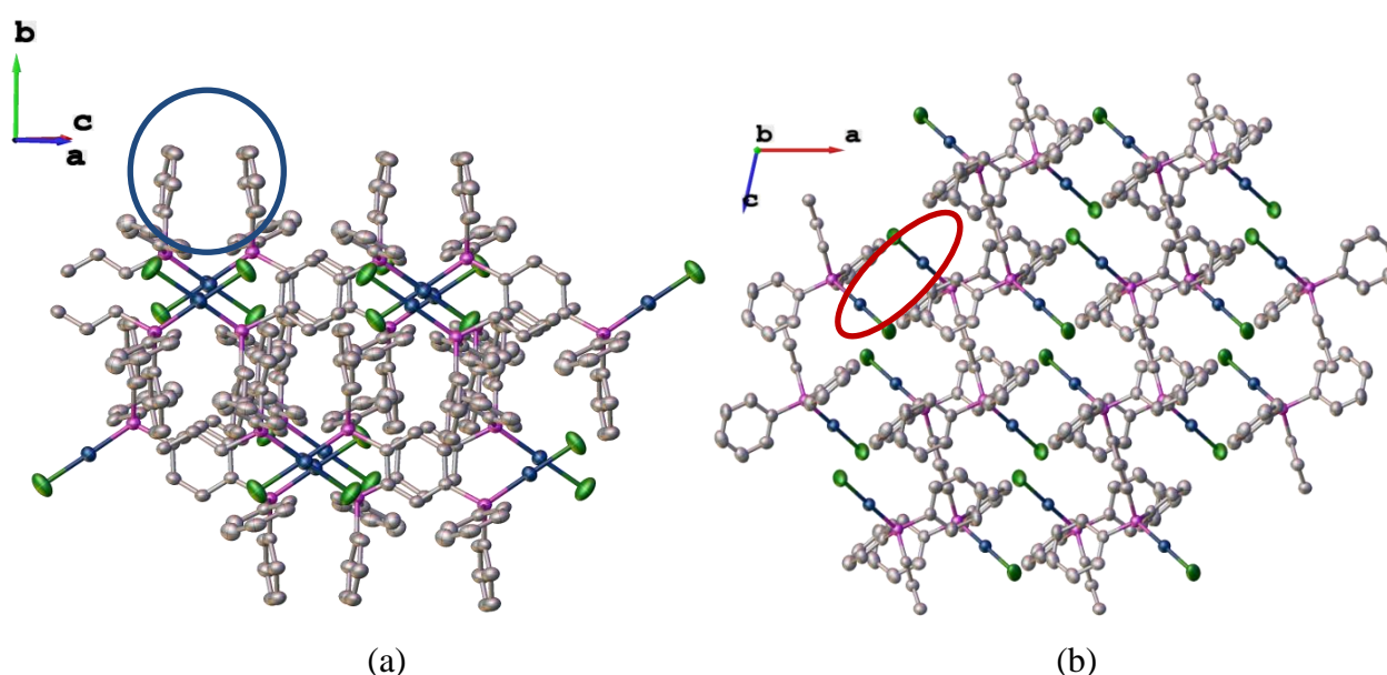
Figure 2. Packing arrangement of 1 at ambient pressure showing (a) \pi\cdots\pi interactions, which are highlighted by a blue circle and (b) aurophilic interactions, which are highlighted by a red ellipse.
