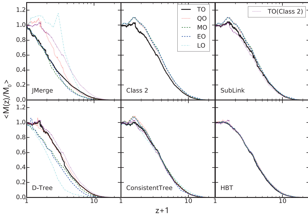
Figure 7. Average mass history for each of the builders as a function of red shift. This corresponds to the total mass in tree main branches for root haloes between 0.5 \times 10^9 M_{\odot} and 1.5 \times 10^9 M_{\odot} at z = 0 , normalized by the mass at z = 0 . Different lines represent merger trees built from different output strategies, as indicated by the legend. Each subpanel displays results for one tree-builder as indicated, except for the four class 2 finders, which are indistinguishable and so are all shown on the same subpanel. The TO line of CLASS2 is reproduced in magenta on all panels for guidance.
