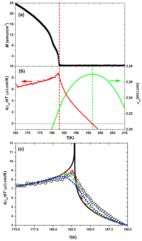
FIG. 2. Simultaneous measurements of (a) the projection of the temperature dependent remanent magnetization along the [1\bar{1}0] easy axis, and (b) the temperature dependence of the resistivity and the temperature derivative of the resistivity ( d\rho_{xx}/dT(T) ), for a 12% Mn 25 nm thick (Ga,Mn)As sample. (c) Calculated results of d\rho_{xx}/dT(T) for power law behavior using the critical exponent from the KF plots with Gaussian broadening \Delta T_C of 0 K (black solid line), 0.5 K (red dashes), 1 K (green short dashes), and 1.5 K (blue dots). Diamond points: the experimental data.
