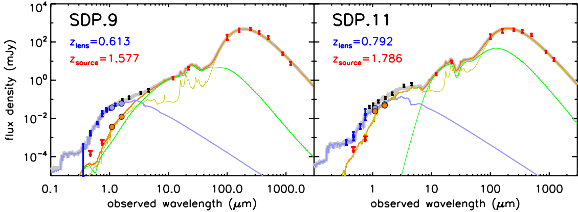
Figure 6. Same as in Fig. 5 for SDP.9 and SDP.11 but with the inclusion of an AGN component, represented by the green curve. The star-forming component, as derived from MAGPHYS , is shown in yellow. The orange curve is the sum of the star-forming and the AGN components.
