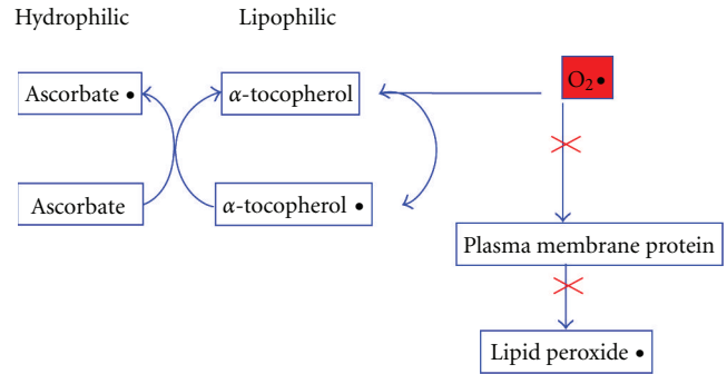
FIGURE 3: Synergistic mechanisms of vitamin C (ascorbate) and vitamin E ( \alpha -tocopherol) to prevent lipid peroxidation. O_2\cdot : oxygen free radical.
