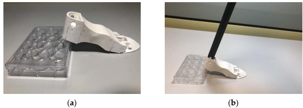
Figure 12. Humanoid foot prototype assembly on a 22 mm step: (a) unloaded test; (b) loaded test.
