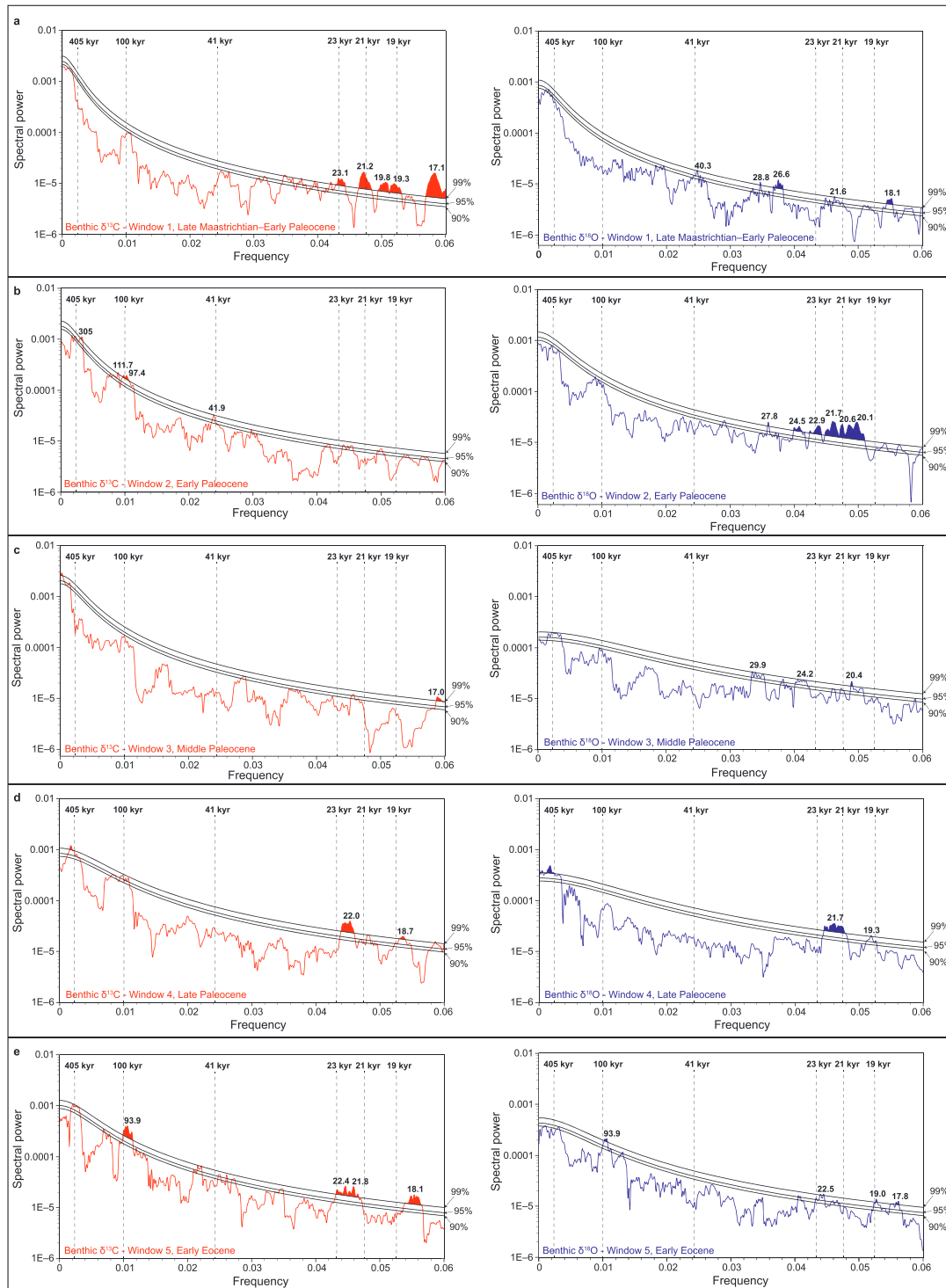
Figure 8. Multitaper Method power spectra for the \delta^{13}C_{\text{benthic}} record (in red) and \delta^{18}O_{\text{benthic}} record (in blue) for the five discrete time windows. (a) Window 1, Late Maastrichtian–Early Paleocene (67.1–64.0 Ma). (b) Window 2, Early Paleocene (64.0–61.25 Ma). (c) Window 3, Middle Paleocene (61.25–58.75 Ma). (d) Window 4, Late Paleocene (58.75–55.93 Ma). (e) Window 5, Early Eocene (55.83–52.35 Ma). Temporal distribution of the time windows is illustrated in Figures 2f and 6g.
