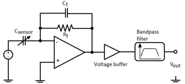
Fig. 8. Schematic of readout circuit for capacitive sensing.
