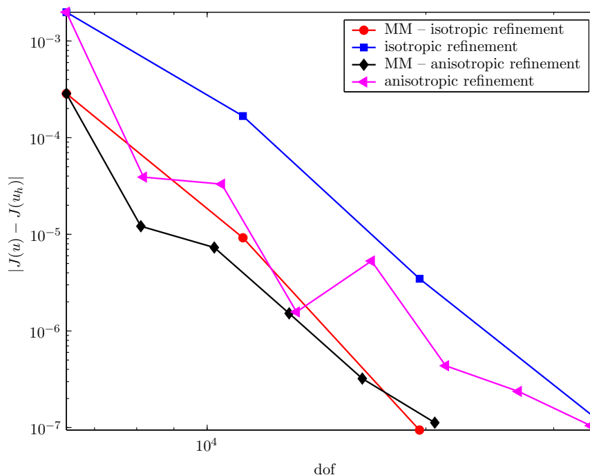
FIGURE 18. Example 3. Meanflow value evaluation. The computed error |J(u) - J(u_h)| versus the total number of degrees of freedom (loglog scale). Comparison between the errors obtained with and without the pre-processing moving mesh strategy.
