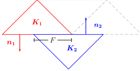
FIGURE 1. A sample of neighboring elements K_1 and K_2 , and their shared face F \in \mathcal{F}_h^I in two-dimensions.
