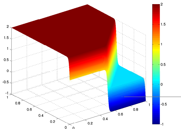
FIGURE 4. Example 1. Elevation plot of the analytical solution u(x, y) = \tanh(60y) - \tanh(60x - 60y - 30) .
