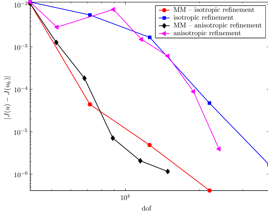
FIGURE 15. Example 3. Point value evaluation. The computed error |J(u) - J(u_h)| versus the total number of degrees of freedom (loglog scale). Comparison between the errors obtained with and without the pre-processing moving mesh strategy.
