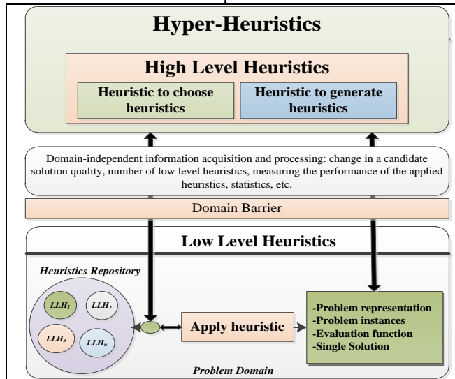
Fig. 2. A generic hyper-heuristic framework [3]
