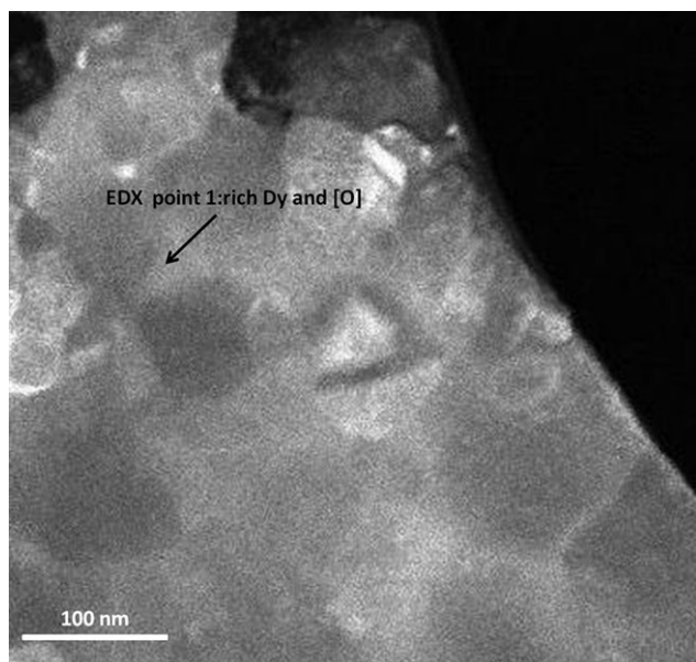
Fig. 5. High-resolution transmission electron microscopy image of suggested \text{Dy}_2\text{O}_3 nucleating agents found in rich Ga area inside the bulk of 3000 ppmw \text{Dy}^{3+} ( \text{DyCl}_3 )-doped \text{Ge}_{16.5}\text{As}_{16}\text{Ga}_3\text{Se}_{64.5} glass. The EDX spectra are shown in Fig. 6 and the corresponding quantified composition is given in Table II.
