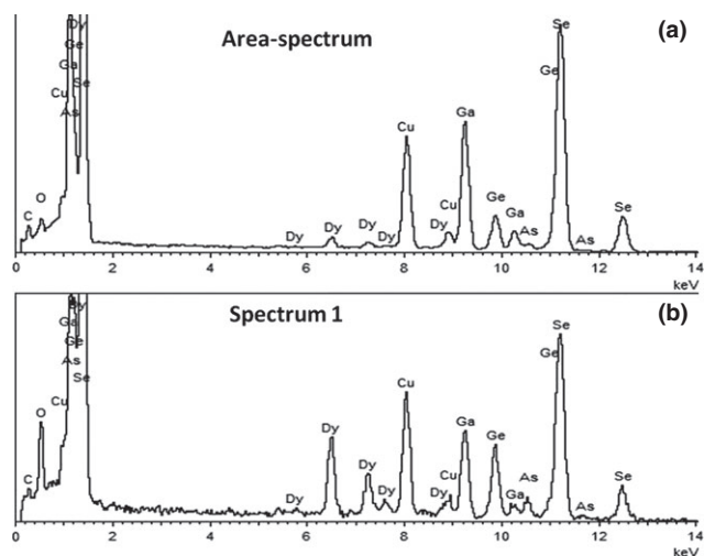
Fig. 6. HRTEM-EDX acquired: (a) area spectrum and (b) point spectrum 1, both from in the bulk of a sample of the 3000 ppmw \text{Dy}^{3+} ( \text{DyCl}_3 )-doped \text{Ge}_{16.5}\text{As}_{16}\text{Ga}_3\text{Se}_{64.5} glass, imaged in Fig. 5. Area spectrum means the HRTEM-EDX spectrum of the whole region shown in Fig. 5, whereas that acquired at a higher resolution to the HRTEM beam itself is referred to as point spectrum 1. The quantified HRTEM-EDX composition results are in Table II.
