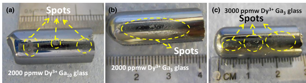
Fig. 7. As-prepared glassmelting results of: (a) 2000 ppmw \text{Dy}^{3+} ( \text{DyCl}_3 )-doped \text{Ge}_{16.5}\text{As}_{16.0}\text{Ga}_{10}\text{Se}_{64.5} glass; (b) and (c): 2000 and 3000 ppmw \text{Dy}^{3+} ( \text{DyCl}_3 )-doped \text{Ge}_{16.5}\text{As}_{16.0}\text{Ga}_3\text{Se}_{64.5} glass, respectively, showing spot defects at the glass surfaces which had been in contact with the silica glass containment during melt cooling and annealing.
