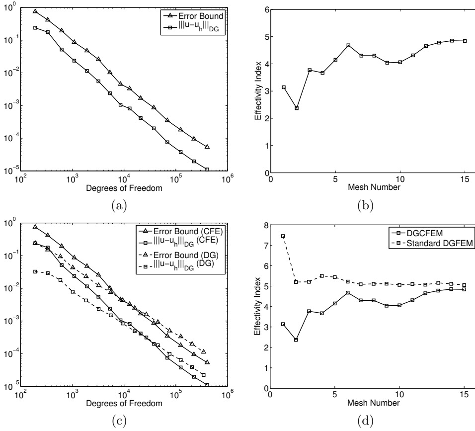
FIG. 6.2. Example 1: Adaptive algorithm employing h -refinement with p = 2 . (a) Comparison of actual and estimated energy norm of the error with respect to the number of degrees of freedom; (b) Effectivity indices; (c) Comparison between DGCfEM and the standard DGFEM (computed without any holes); (d) Effectivity indices for DGCfEM and DGFEM.
