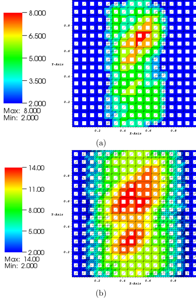
FIG. 6.5. Example 1: Adaptive algorithm employing hp -refinement. hp -Mesh distribution after: (a) 7 adaptive refinements with 416 elements and 4639 degrees of freedom; (b) 16 adaptive refinements, with 2303 elements and 47499 degrees of freedom.
