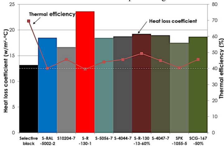
Fig. 2 Impact of colourful coatings/paints on STF thermal performance
