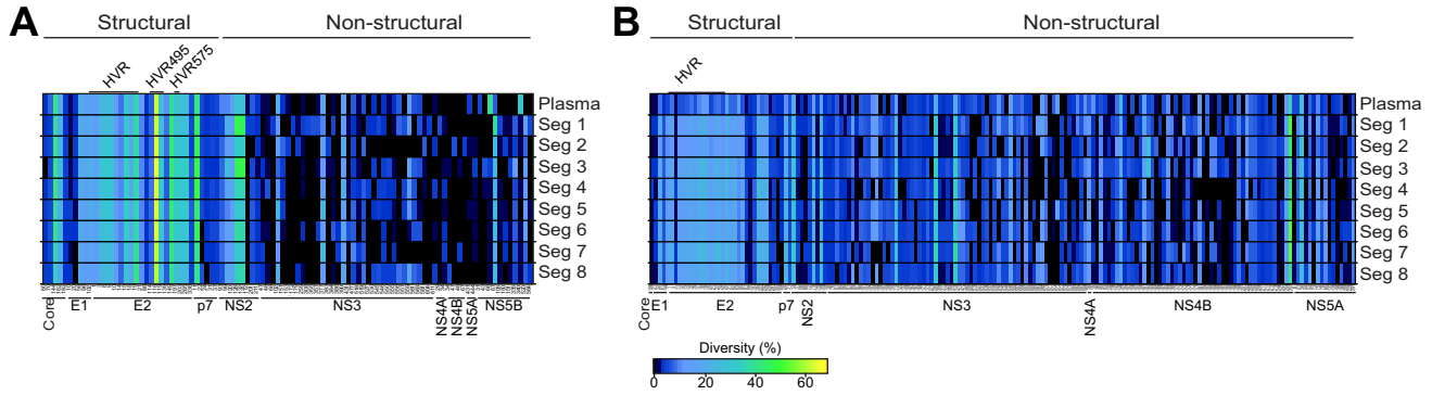
Fig. 3. Deep sequencing of HCV hepatic and plasma quasiespecies. Linear heat map representation of amino acid diversity within the structural and non-structural proteins for the plasma and for the 8 segment biopsies from patient 1 (A) and patient 2 (B). Each square represents a polymorphic codon, coloured to reflect the percentage of reads that exhibit diversity. The diversity scale is colour coded with highly conserved residues in black. Low frequency polymorphisms (<10%) are in dark blue, intermediate levels of polymorphism shade from blue (10%) to green (45%), with the most highly variant residues (45–60%) shaded from green to orange. Only codons exhibiting diversity greater than 1% are shown.
