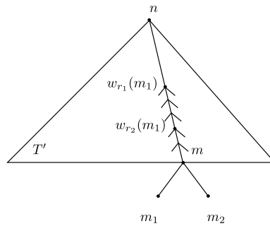
Fig. 2. Tree T and T' = \text{prune}(T, m) .
