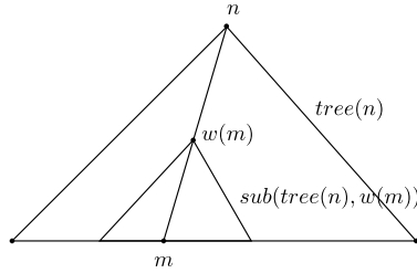
Fig. 4. w(m) of m in tree(n) .
