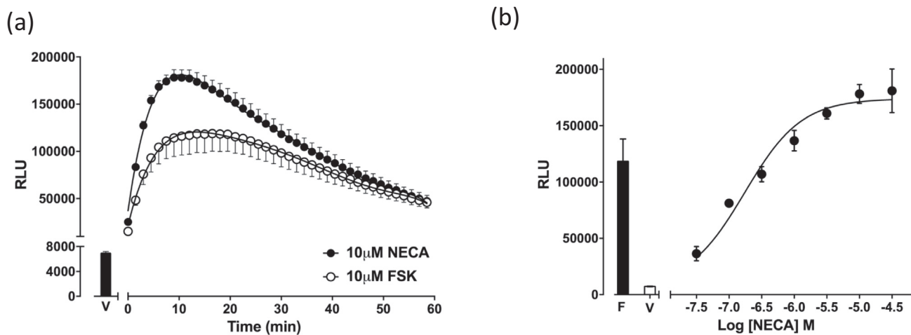
Fig. 1. Forskolin – and NECA – stimulated cAMP Glosensor luminescence. (a) Glosensor luminescence time courses following stimulation by increasing forskolin (10 μM) or NECA (10 μM). Data are mean ± S.E.M. of triplicate determinations obtained in a single representative experiment and expressed as relative luminescence units (RLU). Similar data were obtained in 8 (Forskolin) and 21 (NECA) separate experiments. (b) Representative concentration response curve for NECA obtained from triplicate determinations in a single experiment. Bars show the peak luminescence response to 10 μM forskolin (F) and that seen with vehicle alone (V). Similar data were obtained in 21 separate experiments.
