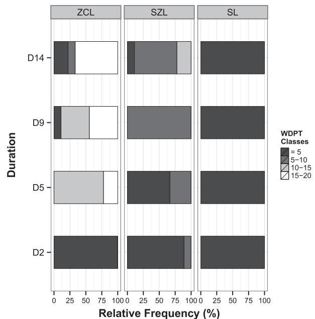
Fig. 5. Relative frequency of four observed water-drop penetration time (WDPT) classes ( < 5 s, 5 s < \text{WDPT} < 10 s, 10 s < \text{WDPT} < 15 s, and 15 s < \text{WDPT} < 20 s) for three soil types (Silty clay loam – ZCL; Sandy silt loam – SZL; Sandy loam – SL) at different rainfall durations (2, 5, 9 and 14 min: D2, D5, D9, D14 respectively).
