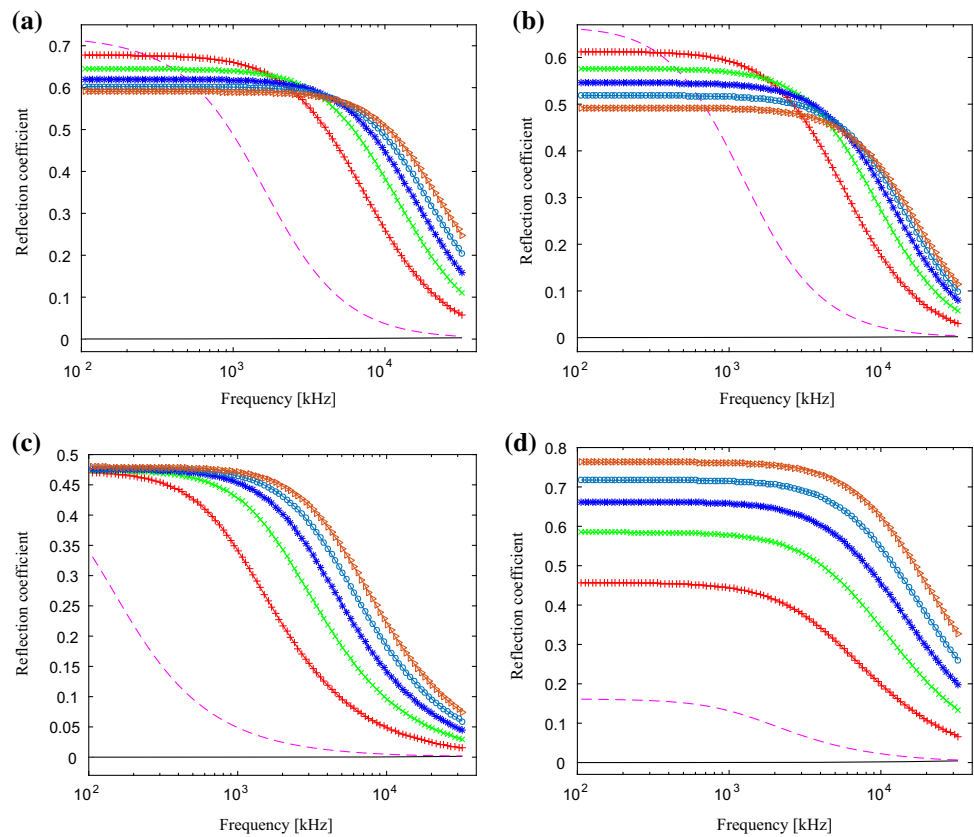
Fig. 20 Wave reflection coefficient magnitude from the 20% (-) width delamination within the sandwich beam: non-pressurised (-), pressure p = 0.01 GPa (- -), 0.1 GPa (-+), 0.2 GPa (-x), 0.3 GPa (-*), 0.4 GPa (-o) and 0.5 GPa (->). a Bending wave about y-axis. b Bending wave about z-axis. c Longitudinal wave. d Torsional wave
