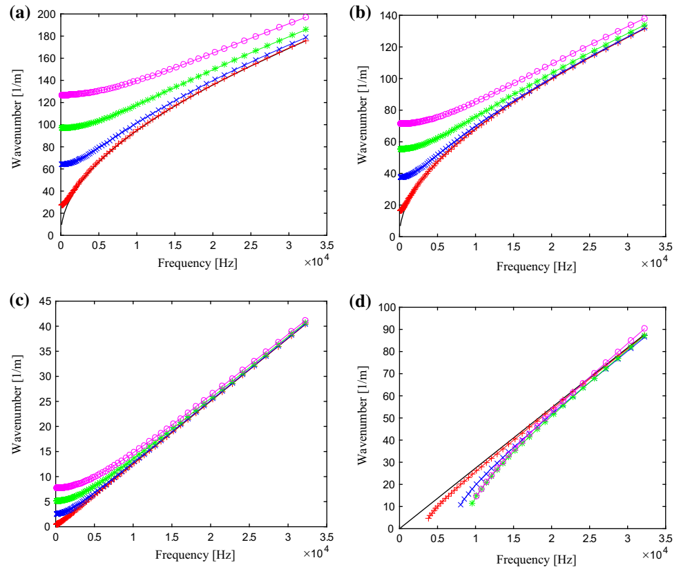
Fig. 14 Dispersion curves for the transversely-isotropic beam: non-pressurised (-), internal pressure p = 0.1 GPa (-+), 0.5 GPa (-x), 1.0 GPa (-*) and 1.5 GPa (-o). a Bending wave about y-axis. b Bending wave about z-axis. c Longitudinal wave. d Torsional wave
