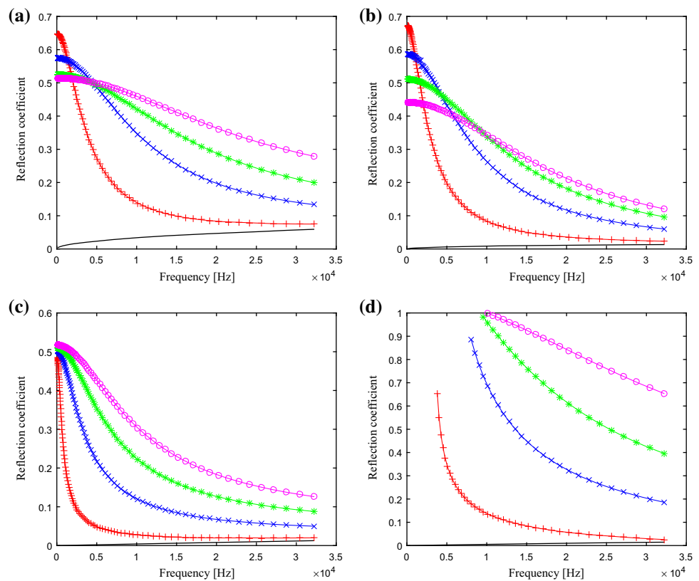
Fig. 15 Wave reflection coefficients for the transversely-isotropic laminate with 20% depth crack: non-pressurised (-), internal pressure p = 0.1 GPa (-+), 0.5 GPa (-x), 1.0 GPa (-*) and 1.5 GPa (-o). a Bending wave about y-axis. b Bending wave about z-axis. c Longitudinal wave. d Torsional wave
