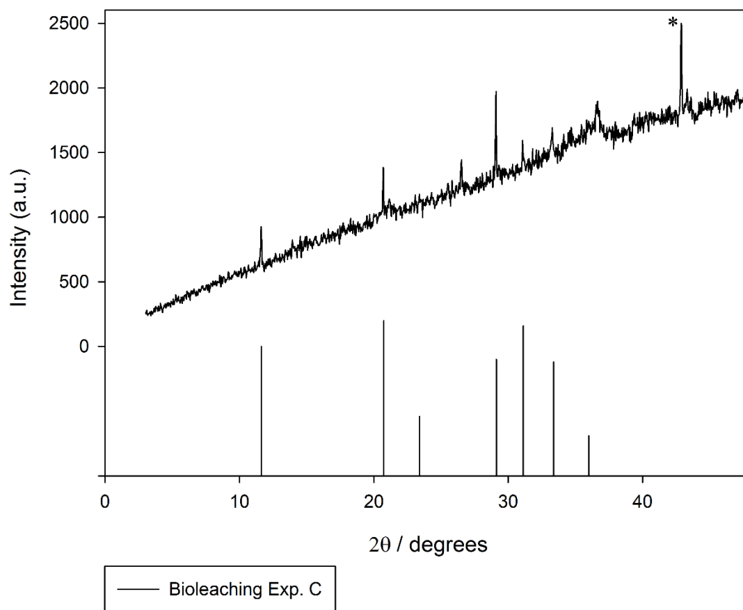
Fig. S2. X-ray powder diffraction pattern for bioleaching sample from Exp. C. The positions of major peaks expected in the range 10 \leq 2\theta / ^\circ \leq 40 for gypsum (black) are shown at the foot of the plot. A single peak from the sample holder is marked with an asterisk.
