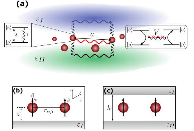
FIG. 1. (a) : A system of N atoms in vacuum is surrounded by one or more layers of metallic or dielectric materials (with dielectric constant \varepsilon_j , with j = I, II, \dots ). Each single atom is described as a two-level system with the excited state |e\rangle decaying to the ground state |g\rangle with a free-space rate \gamma . As the distance between the atoms a becomes comparable to the wavelength of the |e\rangle \rightarrow |g\rangle transition \lambda , the coherent and incoherent scattering of photons gives rise to long-range exchange interactions between the atoms at a rate V . Part of this scattering occurs through coupling to the vacuum radiation field (red) and part through the coupling to the surfaces (black). We study specifically two situations: (b) : the atoms at the same distance z from a surface and (c) : the atoms placed between two identical surfaces.
