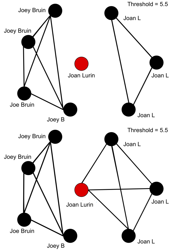
Fig. 6: An example of how refinement is used to improve our clusters. The left figure shows that by removing the record “Joan Lurin”, we obtain the two desired subsets. The right figure shows that “Joan Lurin” is inserted back into the appropriate cluster. Note that we have not changed the threshold value \tau during this process.
