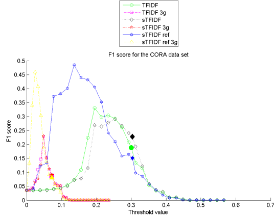
(a) The F_1 score for the Cora data set
