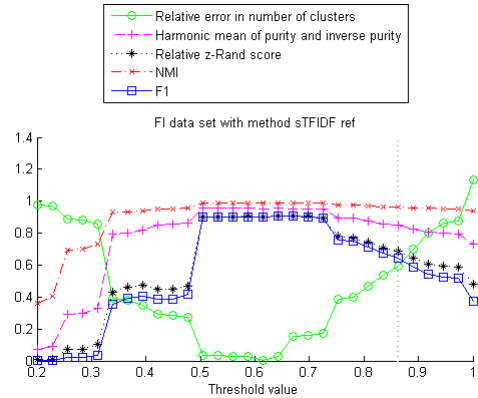
(b) Soft TF-IDF (on word based features) with the refinement step applied to the FI data set
