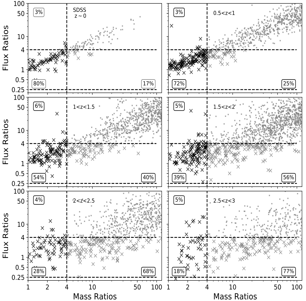
Figure 9. Stellar-mass-ratio vs. H -band flux-ratio for the close-pair systems satisfying our fiducial projected separation (5 – 50 kpc) and redshift proximity choices for SDSS ( \Delta v_{12} \leq 500 \text{ km s}^{-1} ; z \sim 0 ; top left) and CANDELS (B09; 0.5 \leq z \leq 3 ; rest of the panels). We show the pairs that satisfy our fiducial mass-ratio criterion ( 1 \leq M_1/M_2 \leq 4 ) in large-black points, those having a M_1/M_2 > 4 but satisfy the flux-ratio criterion ( 1 \leq |F_1/F_2| \leq 4 ) in large-grey points, the remaining points in small-grey markers. To visualize the contamination from minor pairs ( M_1/M_2 > 4 ), introduced by the flux-ratio criterion in each redshift panel, we show the percentage of pairs that satisfy either mass-ratio or flux-ratio selection that fall in each of the three quadrants. We notice that the contamination increases steadily from z \sim 0 to z = 3 , causing inflated f_{\text{mc}} values observed in Figure 8 (see § 4.3 for discussion).
