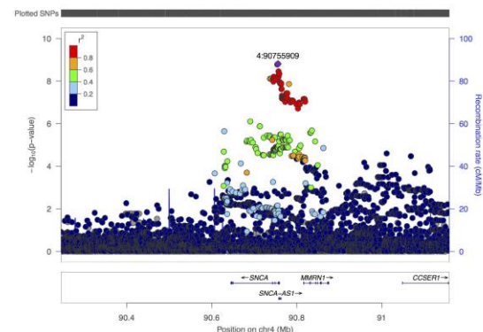
Figure 4: Regional association plot for the SNCA locus. Purple represents rs1372517, which is the most associated SNP at the locus also present in the 1000Genomes dataset. The variant rs1372517 is in complete LD with rs7681440. Colours represent LD derived from 1000Genomes between each variant and the most associated SNP.
