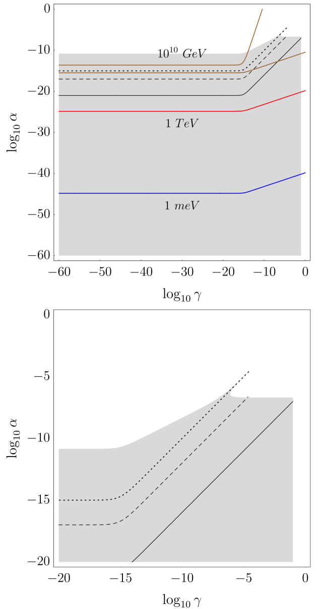
FIG. 2: Same as Fig. 1 but for \beta = 10^{-15} .
