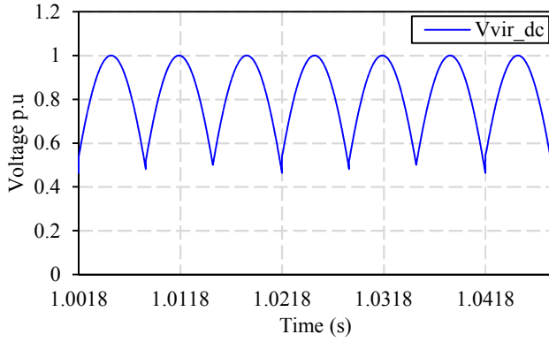
Fig. 5 The virtual DC voltage wave. Voltage in p.u. where the base voltage is V_{base}=220V .
