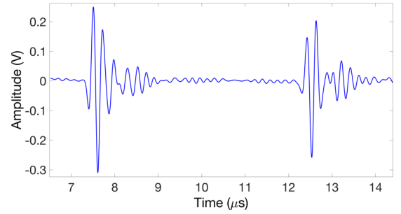
Fig. 5. The pulse echoes with 5 MHz center frequencies from reflections at the top left of back wall of a corroded sample after 301 mins of corrosion.
