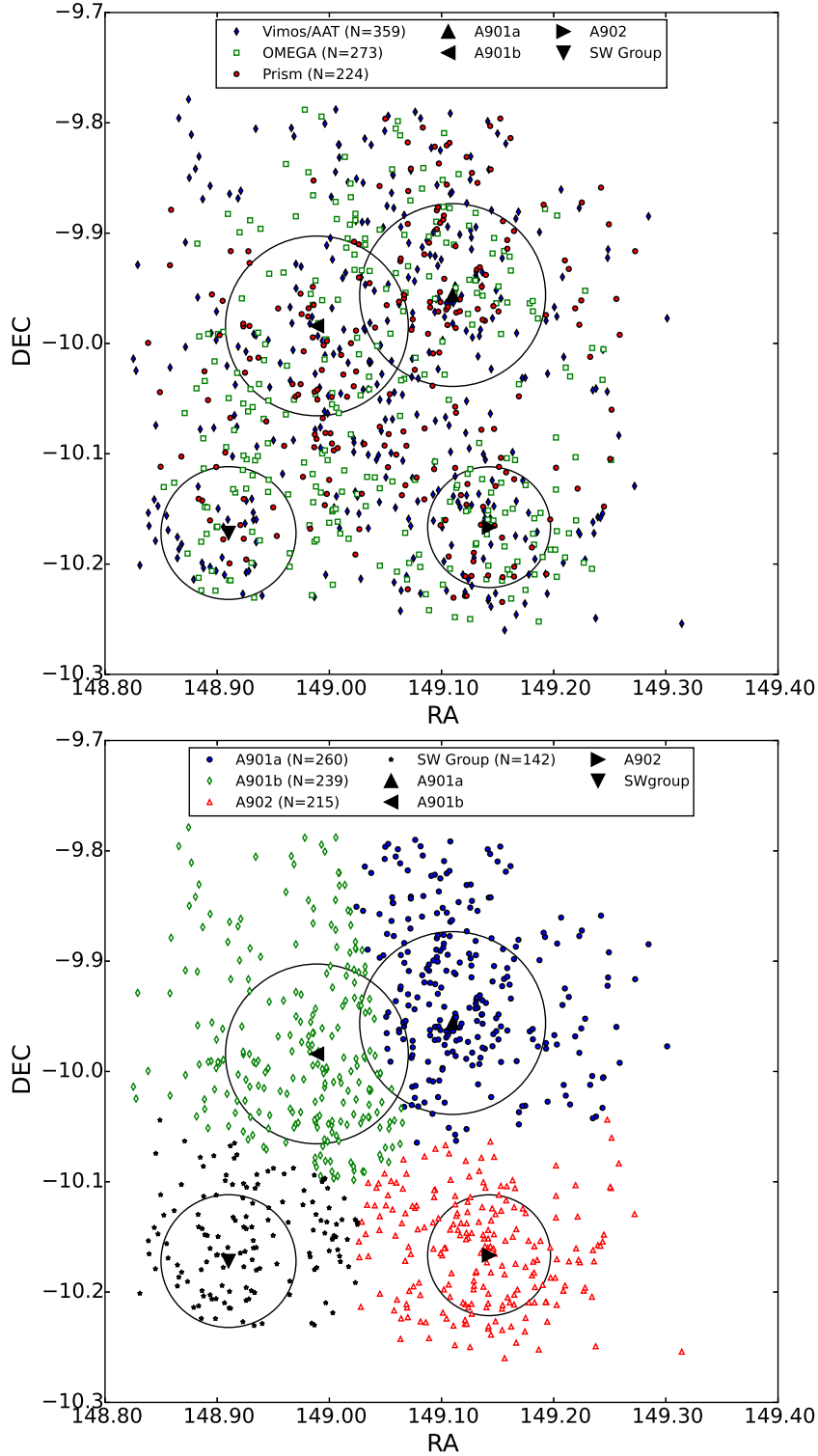
Figure 5. The top panel shows the spatial distribution of the 856 galaxies in sample S2 coded by the source of the adopted redshifts. The four subclusters are separately labelled, and their spheres of influence ( R_{200} ) are shown as circles. In the bottom panel, galaxies are colour coded by the nearest cluster centre.
