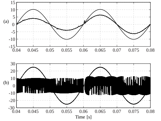
Fig. 8. Simulation results of the proposed method in transient state (Method II): (a) source voltage v_{sA} [V/25] and source current i_{sA} [A]; (b) capacitor voltage v_A [V/10] and input current i_A [A].
