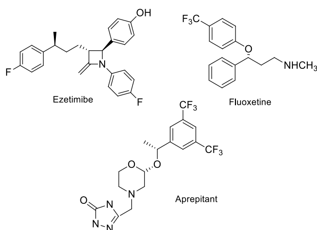
Fig. 1 Examples of drugs derived from chiral aromatic secondary alcohols precursors.
