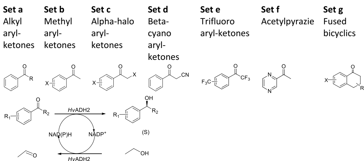
Fig. 3 Various aromatic ketones derivatives and general scheme of their reduction with HvADH2 .
