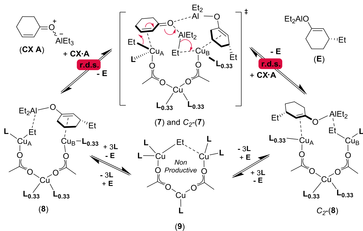
Scheme 3. Mechanism for \text{Cu}^{\text{I}}/\text{L} 1,4-addition of \text{AlEt}_3 ( A ) to cyclohex-2-en-1-one ( CX ) consistent with all experimentally observed data herein. The presence of any metal-coordinated solvent is excluded for clarity; \text{L}_{0.33} indicates partial (33%) binding to that site. 22 Each catalytic cycle interconverts \text{Cu}_\text{A} with \text{Cu}_\text{B} and their respective roles within the cycle.
