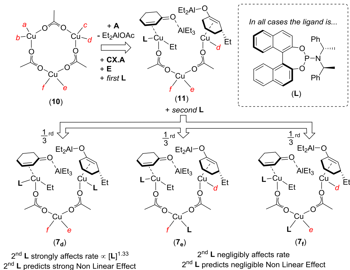
Scheme 3. Mechanism for \text{Cu}^{\text{I}}/\text{L} 1,4-addition of \text{AlEt}_3 ( A ) to cyclohex-2-en-1-one ( CX ) consistent with all experimentally observed data herein. The presence of any metal-coordinated solvent is excluded for clarity; \text{L}_{0.33} indicates partial (33%) binding to that site. 22 Each catalytic cycle interconverts \text{Cu}_\text{A} with \text{Cu}_\text{B} and their respective roles within the cycle.
