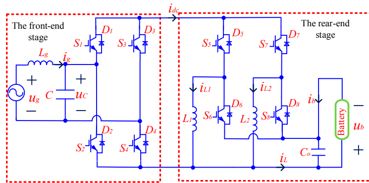
Figure 1. The presented bidirectional converter topology.
