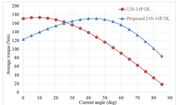
Fig. 10 Average torque versus current angle
