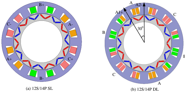
Fig. 1 Conventional winding layouts for 12slots/14poles machine (a) Single layer (b) Double layer
