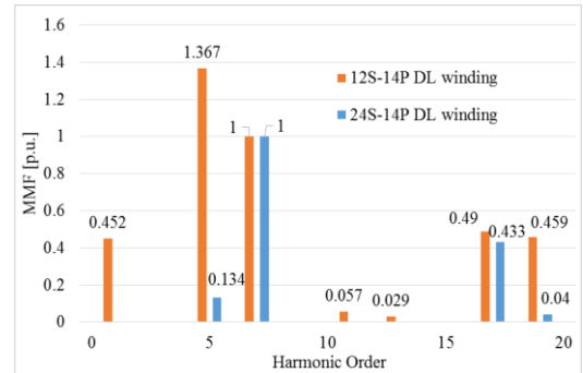
Fig. 6 MMF distribution of two winding layout
