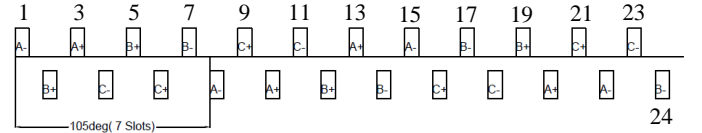
Fig. 5 Concept of “stator shifting” based on a 24 slot 14 pole machine
