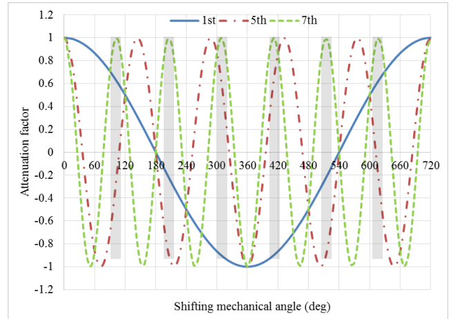
Fig. 4 Attenuation factor for different order MMF harmonics
