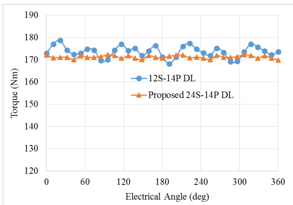
Fig. 8 Comparison of torque performances between two machines
