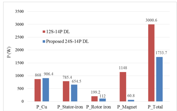
Fig. 9 Comparison of output performances between two machines
