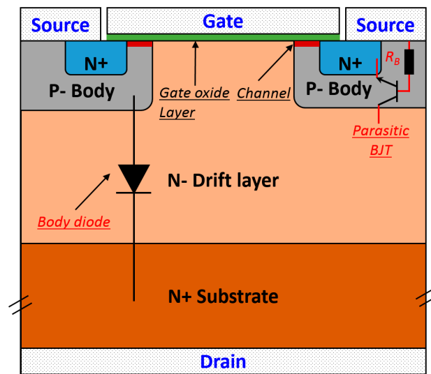
Figure 1. Structure of an N-channel power MOSFET.
