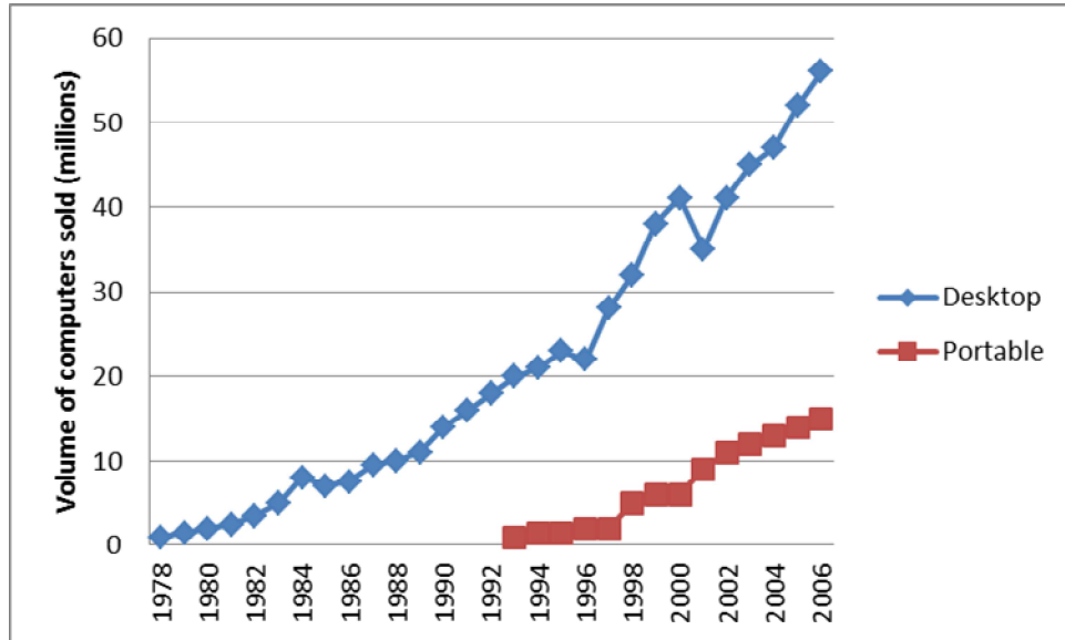
Figure 1. Sales Data on Desktop and Portable Computers (1978 – 2006).
