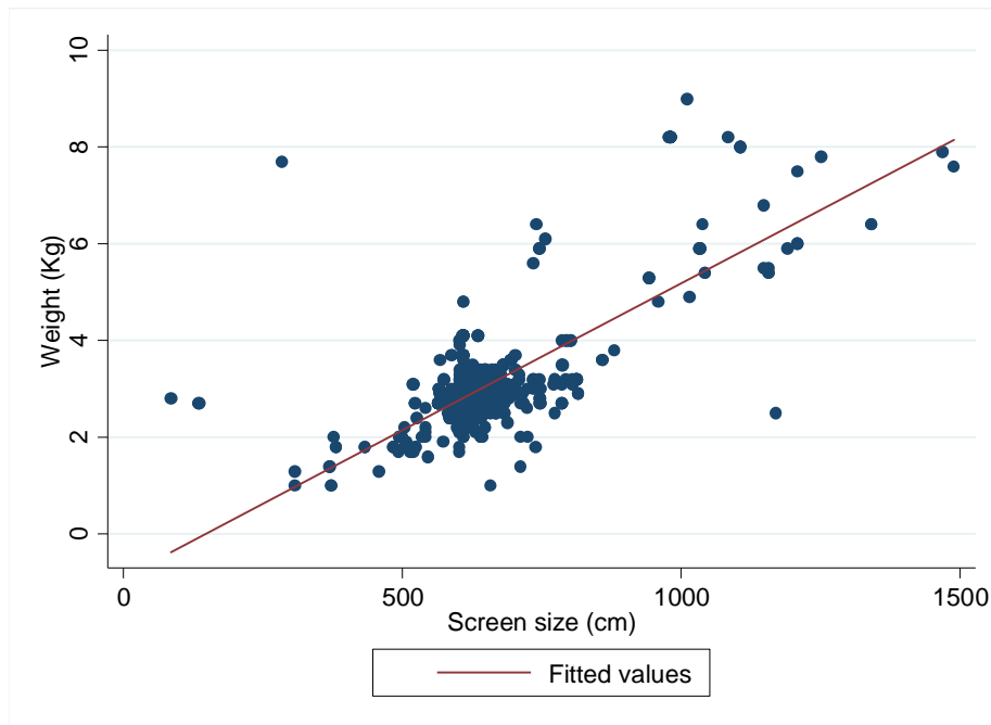
Figure 2. Scatter Plot of Weight against Screen Size, with Fitted Prediction Line
