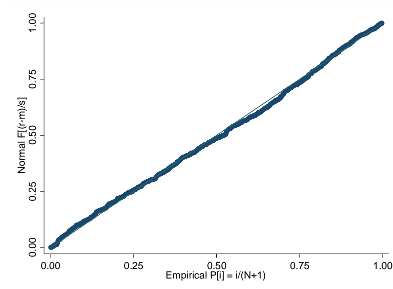
Figure 4a. Standardized Normal Probability Plot of Model 3 Residuals.
