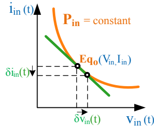
Fig. 4: Characteristic curve of the ideal CPL
