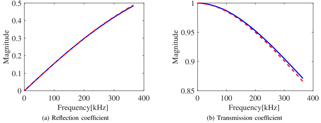
Fig. 5. Wave interaction coefficients for a finite joint connecting two bars: analytical(-), WFE-FE(- -)
