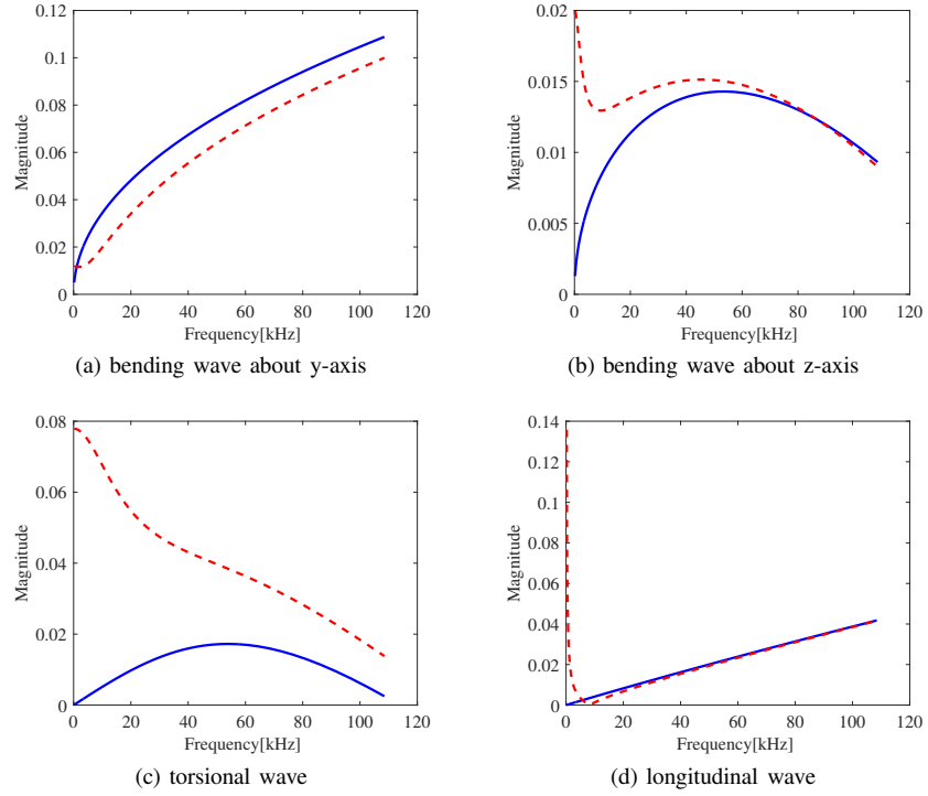
Fig. 7. Wave reflection coefficient magnitude for the 20% depth cracked coupling joint: non-pressurised (-), pressurised (- -) monolithic laminates
