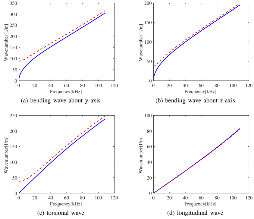
Fig. 8. Dispersion curves for the non-pressurised (-) and 1 GPa pressurised (- -) composite laminates
