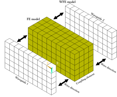
Fig. 2. Periodic structure comprising of two waveguides and a coupling element
