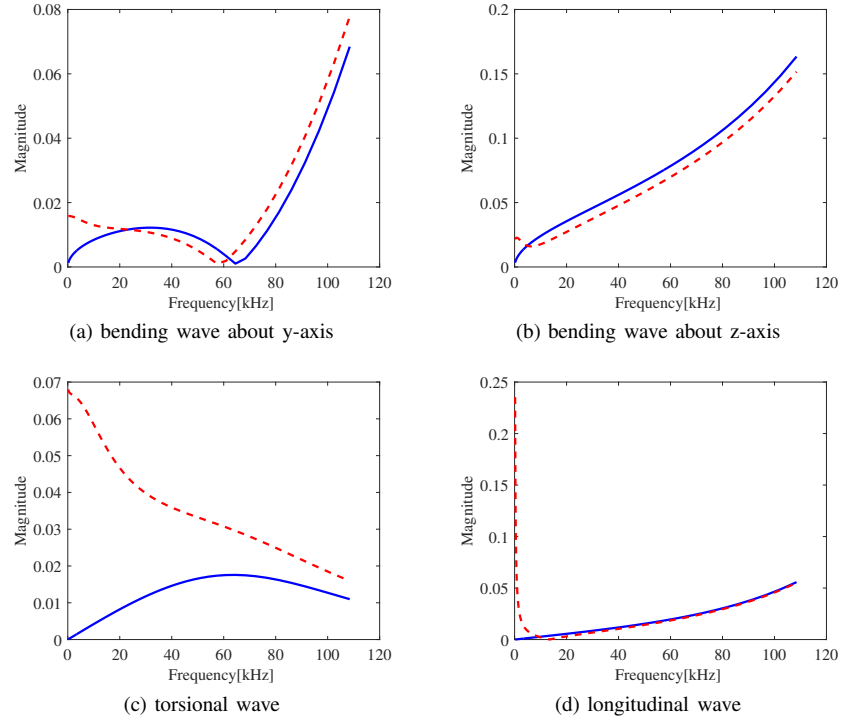
Fig. 9. Wave reflection coefficient magnitude for the 0.002m depth cracked coupling joint: non-pressurised (-) and pressurised (- -) composite laminates
