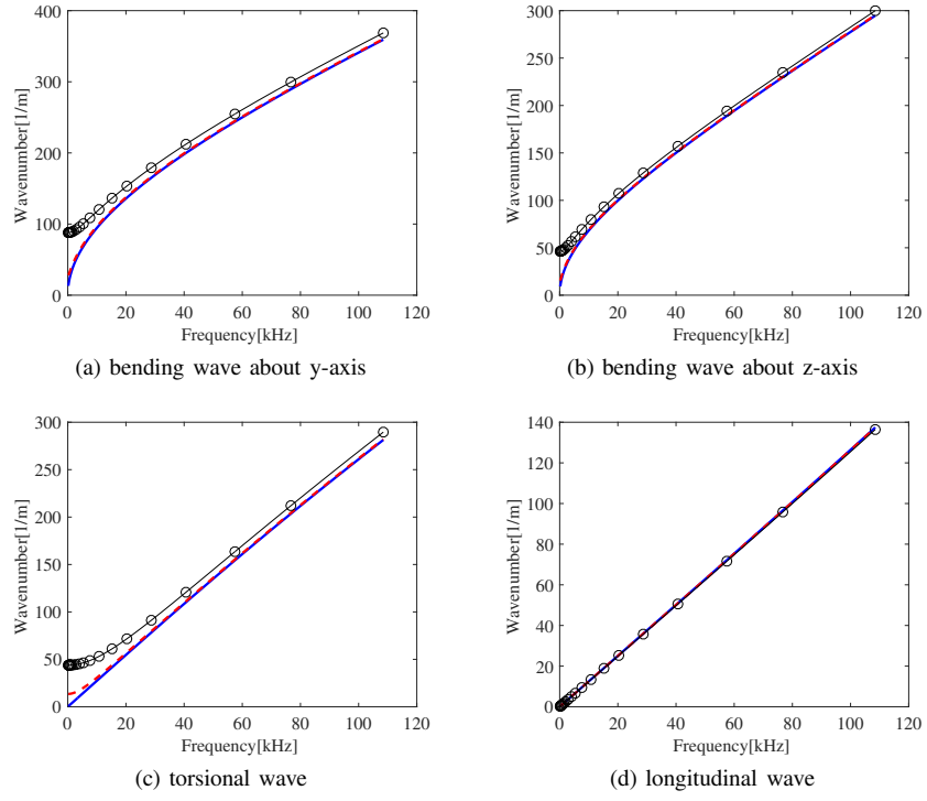
Fig. 6. Dispersion curves for the non-pressurised (-), 100 MPa (- -) and 1 GPa (-·-) pressurised monolithic laminate
