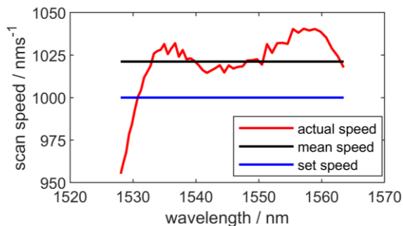
Figure 5. Comparison of tuneable laser wavelength scan rate for a setting of 1000 \text{ nm s}^{-1} .
