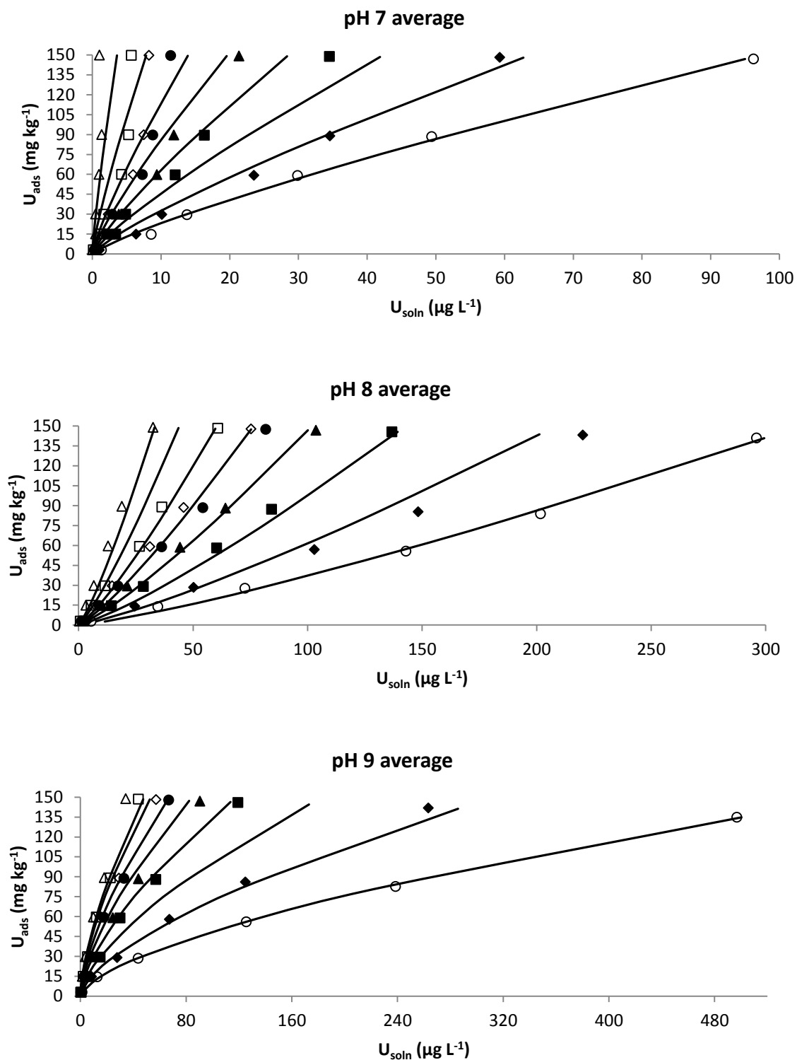
Figure 4: Time-dependent adsorption isotherms for U^{VI} on biochar for equilibration times (days) of: zero (•), 1 (♦), 2 (■), 3 (▲), 4 (●), 5 (◇), 7 (□), 15 (△). Instantaneous adsorption (•) was estimated from the 'zero time' Freundlich isotherm parameters (Figure 3); the model lines shown were calculated from average values of the reversible first-order kinetic model parameters k_a and k_b .
