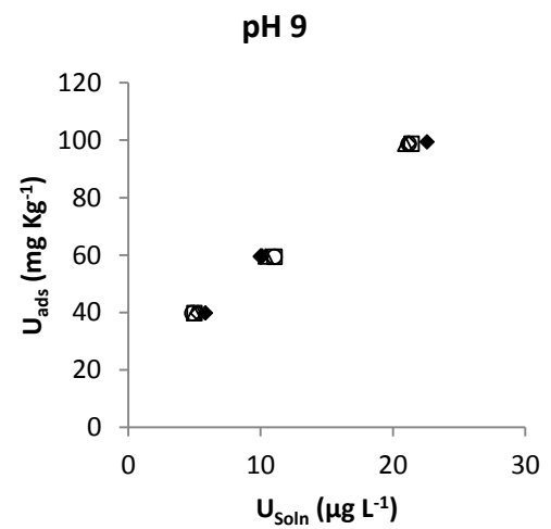
Figure 6: Uranium ( U^{VI} ) desorbed from biochar at different pH values; \blacklozenge = adsorption (15 days), and desorption \diamond = 1 day, \triangle = 2 days, \square = 3 days and \circ = 4 days.
