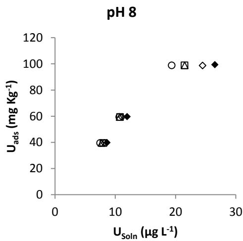
Figure 6: Uranium ( U^{VI} ) desorbed from biochar at different pH values; \blacklozenge = adsorption (15 days), and desorption \diamond = 1 day, \triangle = 2 days, \square = 3 days and \circ = 4 days.
