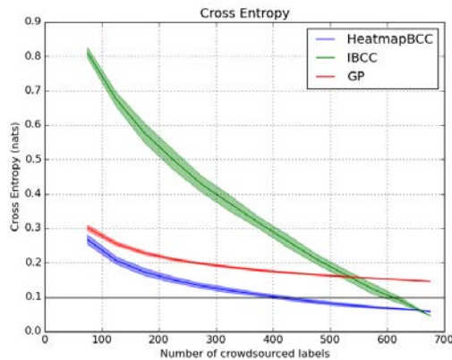
Figure 6: Cross entropy error for Bayesian heatmaps (HeatmapBCC), a Gaussian process density estimator (GP) and independent Bayesian classifier combination (IBCC), evaluated against IBCC predictions with 675 reports on a 100 \times 100 grid. Shaded areas to either side show standard deviation over 20 repeats with different subsets of the data.
