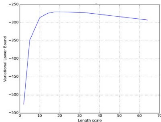
Figure 4: Model evidence variational lower bound for our Bayesian heatmap model learned with different length-scales on Haiti UNOSAT building damage assessment data(Corbane et al., 2011).
