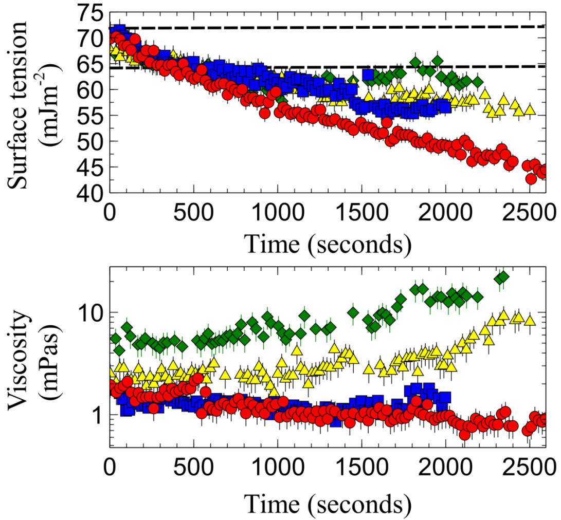
Figure 3. Time dependence of the surface tension (top panel) and viscosity (bottom panel) of evaporating glycerol/water solutions. Data are shown for four droplets of similar size having initial compositions of 1wt% (red circles), 5wt% (blue squares), 25wt% (yellow triangles) and 50wt% (green diamonds) of glycerol. The initial compositions correspond to glycerol volume fractions of 0.008, 0.04, 0.209 and 0.44 respectively. The dashed horizontal lines in the top panel correspond to the surface tensions of pure water and pure glycerol respectively
