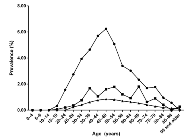
Fig. 1. Age-specific prevalence of schizophrenia in individuals with a first-degree (circle), or second-degree (square) relative with schizophrenia and in the general population (triangle) in Taiwan in 2013.
