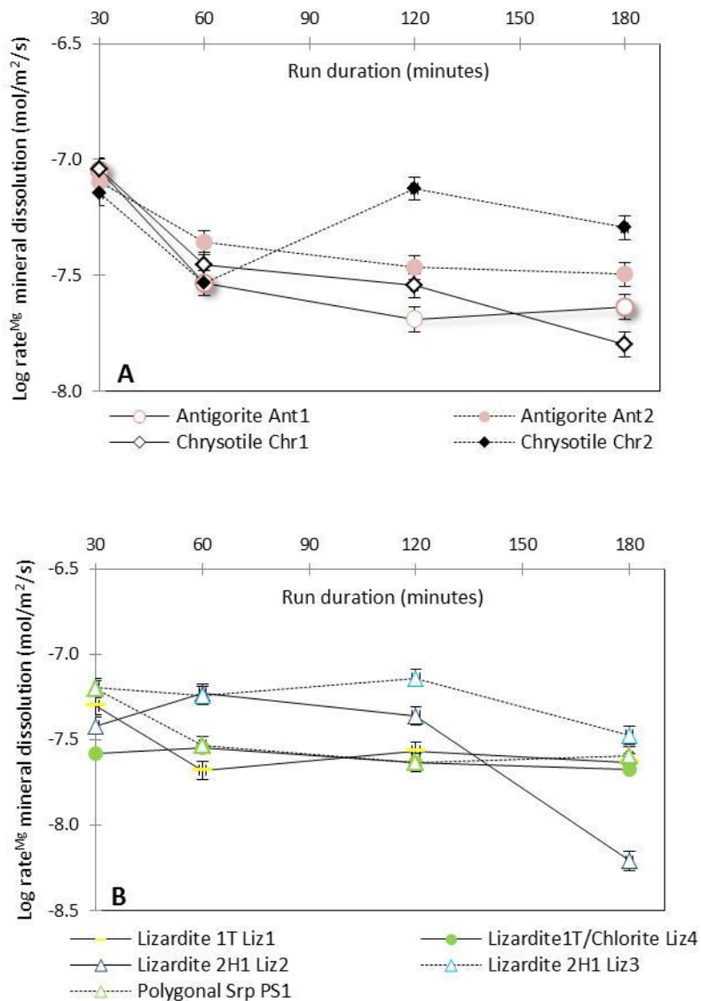
Figure 5 The log rate (logR Mg ) of mineral dissolution as a function of time: A) showing antigorite Ant1, Ant2, and chrysotile samples Chr1, Chr2; B) showing lizardite samples Liz1 1T , Liz2 2H1 , Liz3 2H1 , Liz4 1T and the polygonal serpentine sample PS1. The rates were calculated based on the concentrations of Mg in the leached solutions and normalised for changes in mineral stoichiometry. It is clear that lizardite 2H 1 and chrysotile exhibited higher values of logR Mg than antigorite and Liz1 1T , PS1; largely corresponding to the degree of mineral dissolution illustrated by the Mg EE .
