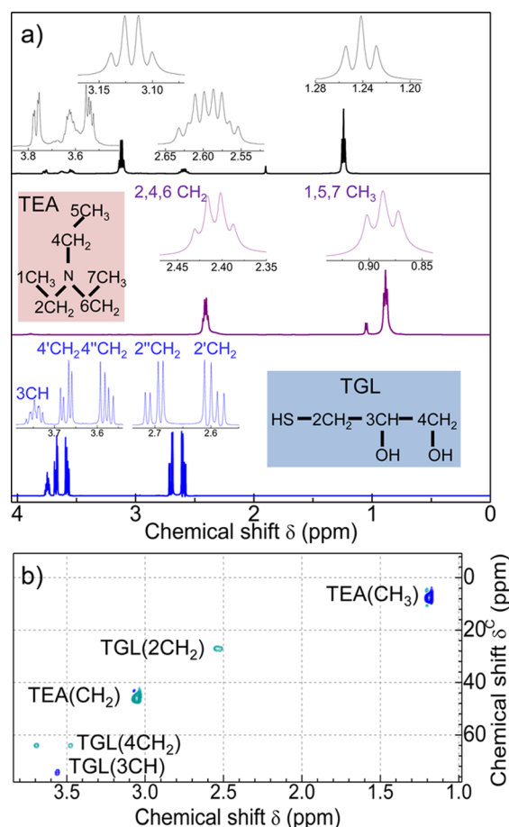
Figure 2. (a) ^1H NMR spectra for solutions of undoped PbS QDs (top panel), free TEA (middle panel), and free TGL molecules (bottom panel). Insets are skeletal formulas for TGL and TEA. (b) HSQC spectra of TGL and PbS QDs. The peaks assigned to the CH groups of TEA and TGL molecules for the PbS QDs are indicated. The different color tone is used to distinguish between odd and even CH groups.
