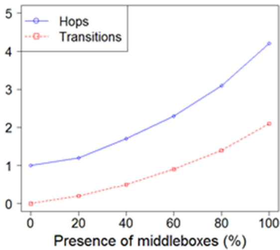
FIGURE 16. End-to-end number of transitions.
