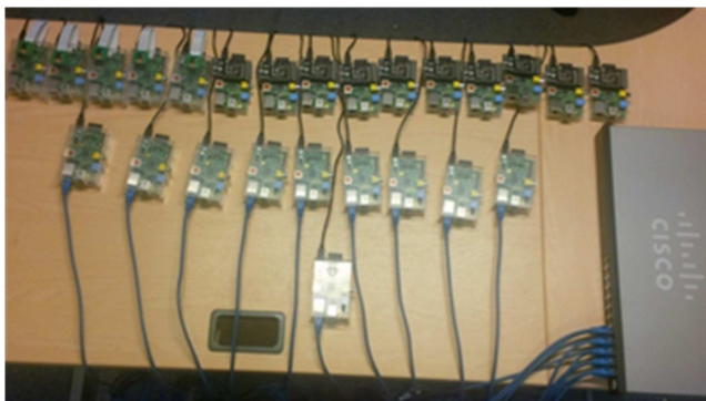
FIGURE 3. A hierarchical architecture Raspberry PI sensor network example.
